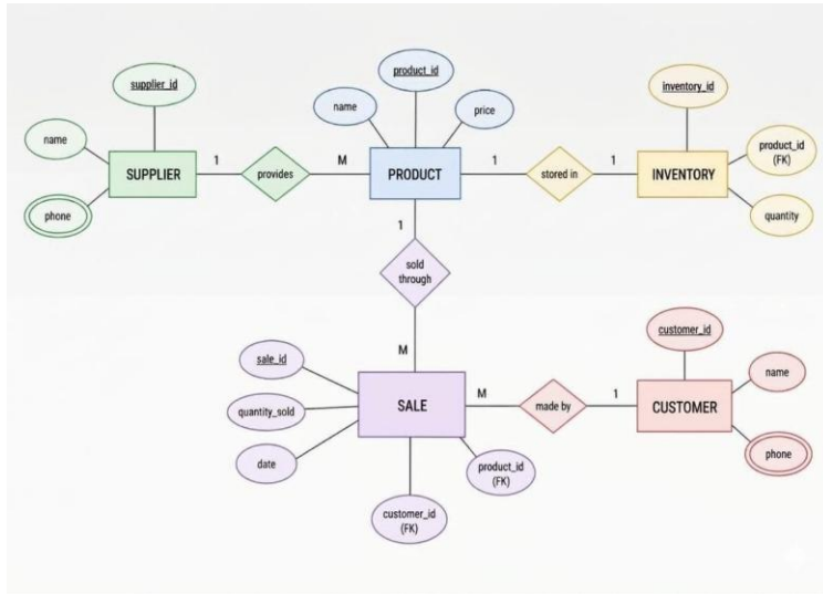
Diagram 1: ER diagram of the inventory system
