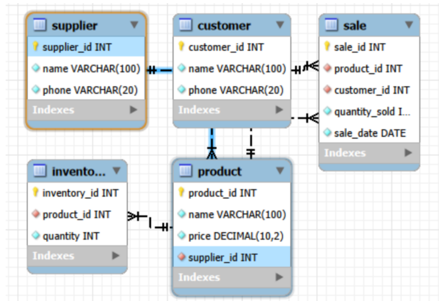
Diagram 2: EER diagram of the inventory system
